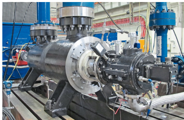
After a Sulzer retrofit, pumps are performance tested at one of Sulzer's test beds (here a third party BB5 pump).
