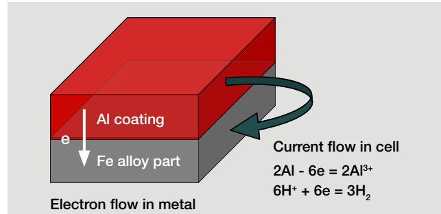
Figure 1: Cathodic protection
