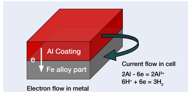
Figure 1: Cathodic protection
