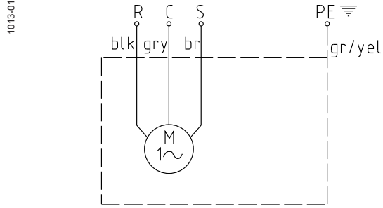
Figure 8: Câblage monophasé
