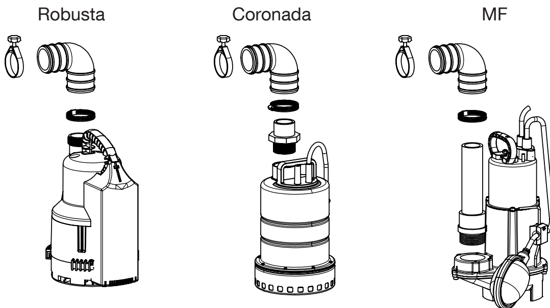
Figure 3: Nirolift pump fitting instructions
