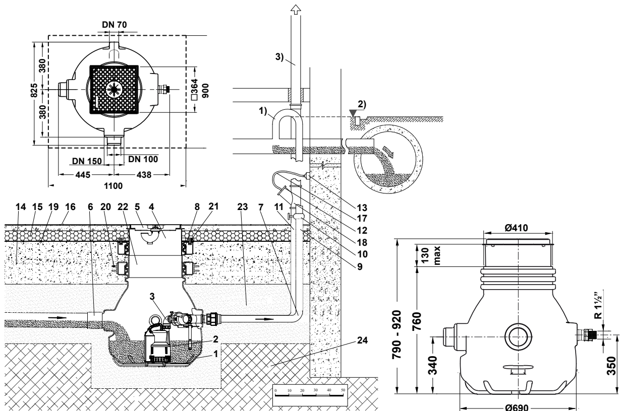
Figure 2: Sanisett installation example and dimensions with DPC connection and Frank Seal kit
