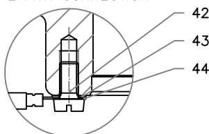
EARTH CONNECTION
