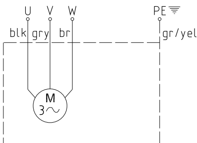
Figure 3 Câblage triphasé
