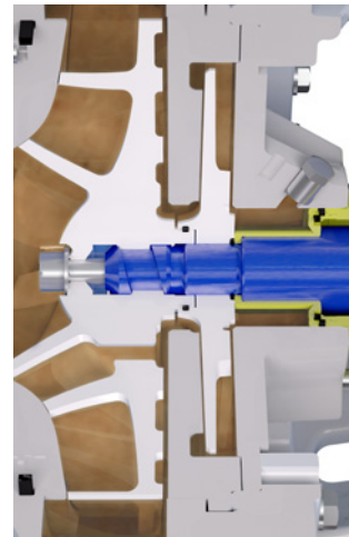
Sulzer dynamic seal stopped
