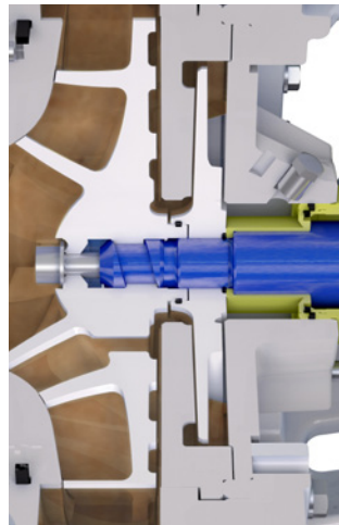
Sulzer dynamic seal running
