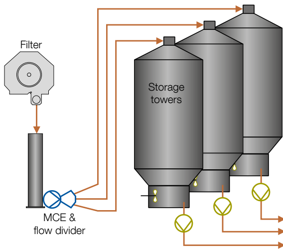
Fig. 10. MC flow divider feeding storage towers.
