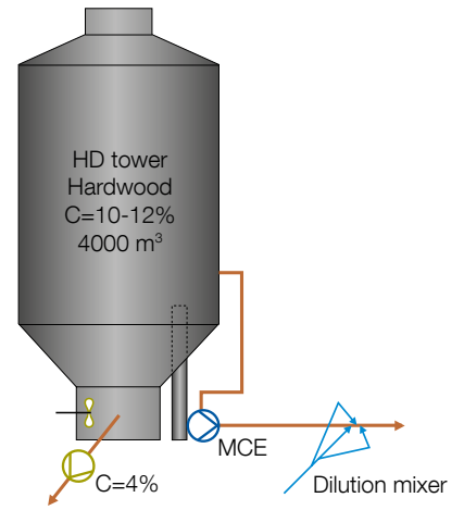
Fig. 24. MC parallel pumping system process application.
