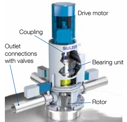
Fig. 21. MC discharger, vertical installation.
