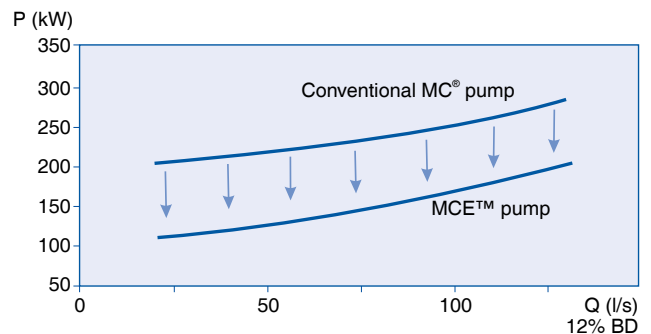
Fig. 1a. Power consumption savings.
