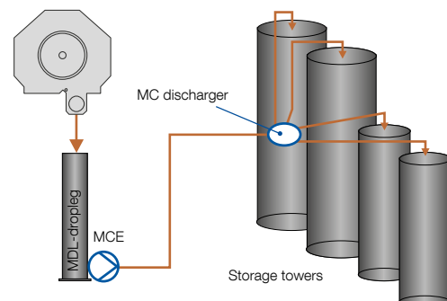
Fig. 19. MC discharger in storage tower application.
