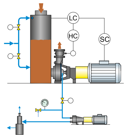
Fig. 8. Control system in MC dropleg installation.
