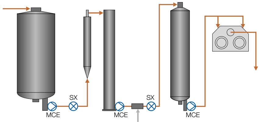
Fig. 13. Typical tower discharge MC pumping systems.
