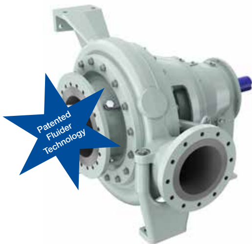
Fig. 3. MCE pump arrangement for the 8 to 18% consistency range.
