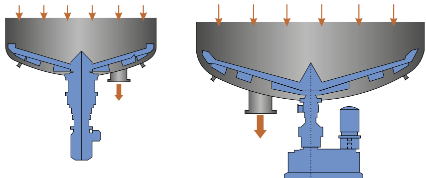
Fig. 15. MC discharge scraper constructions.
