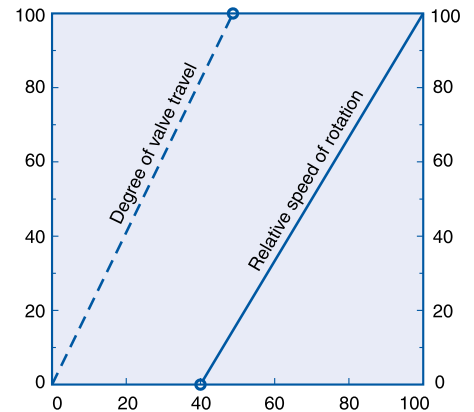
Fig. 7. Combined valve and speed control system.
