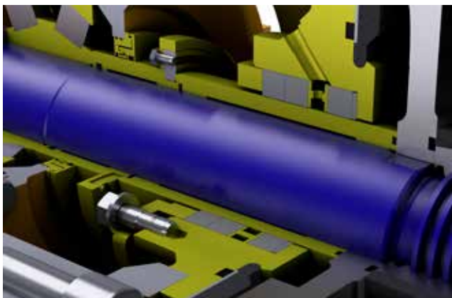
Release collar allows quick and easy removal of the impeller (from size 200).
