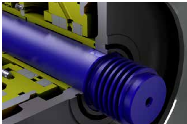
Engagement of expeller and shaft by means of machined surfaces – no key required (from size 100).
