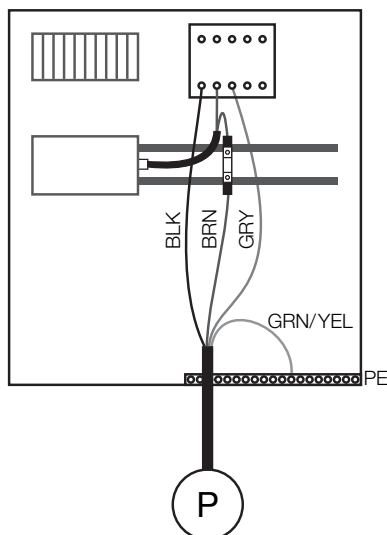
Fig 4. 1~ 1 pump
