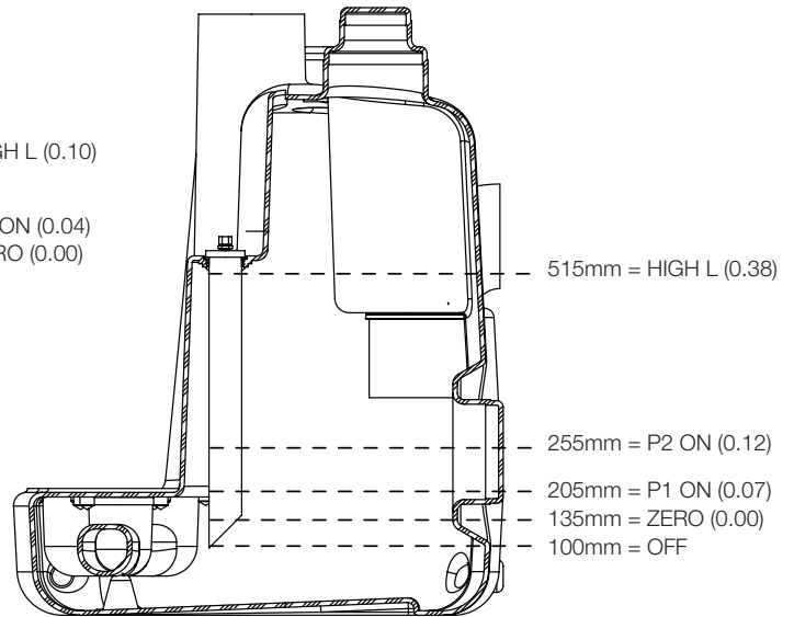
Sanimat 2002
