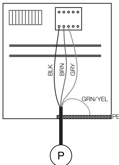
Fig 5. 3~ 1 pump
