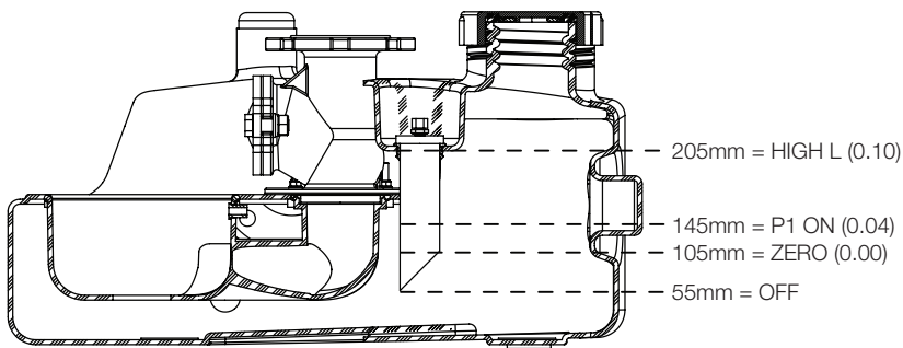
Sanimat 1000
