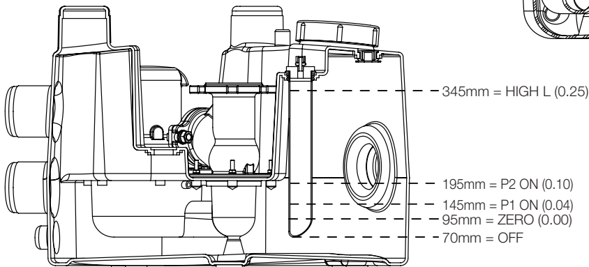
Sanimat 1002
