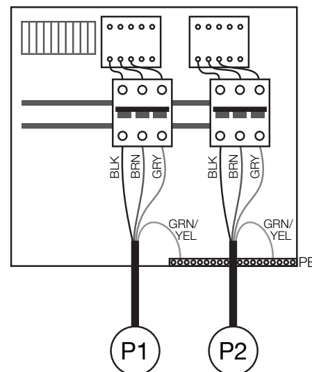
Fig 6. 3~ 2 pump
