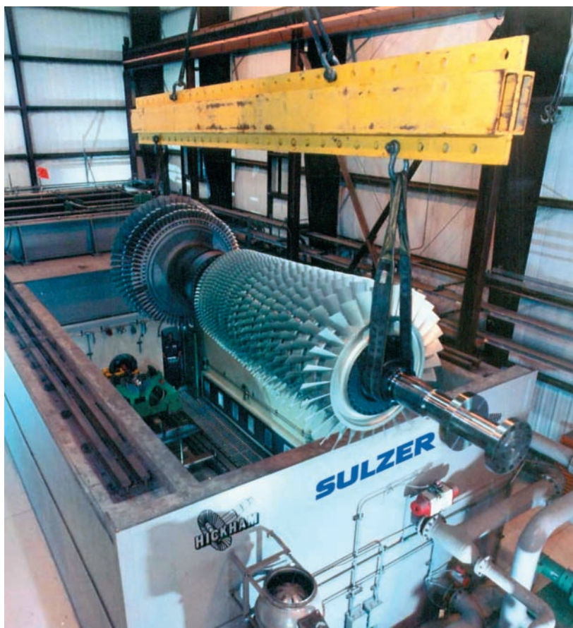
5 Gas turbine rotor assembly being loaded into the bunker. The compressor and turbine sections being bolted together.
