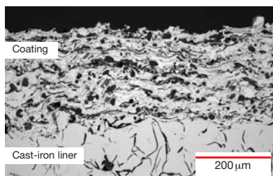
6 Metallographic section of a corrosion resistant MMC coating for heavy-duty diesel applications (as sprayed).
