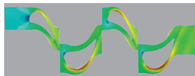
Mach number plots from the CFD analysis of the steam path flow.
