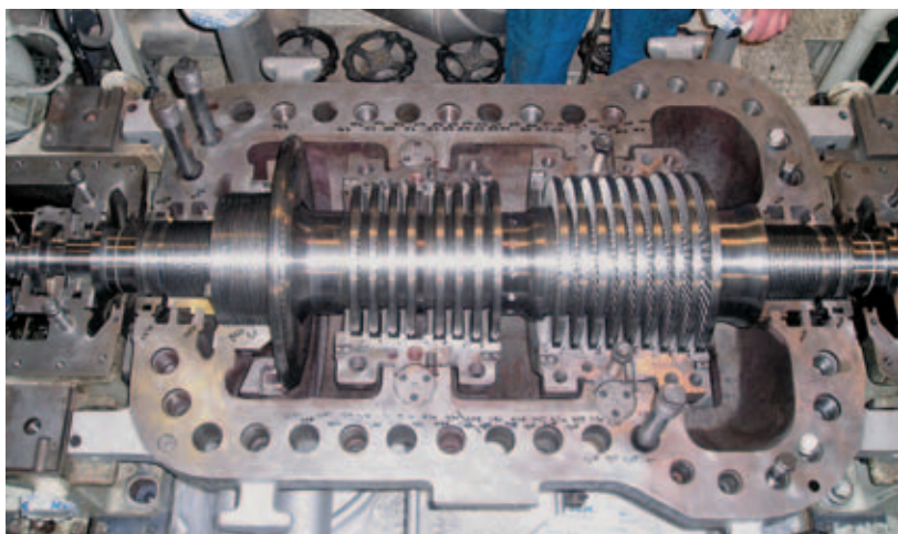
Steam turbine rotor installed within the casing.
