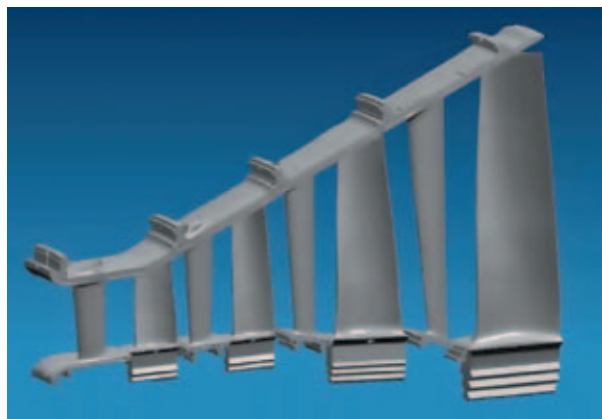
CAD view of the hot gas path section.
