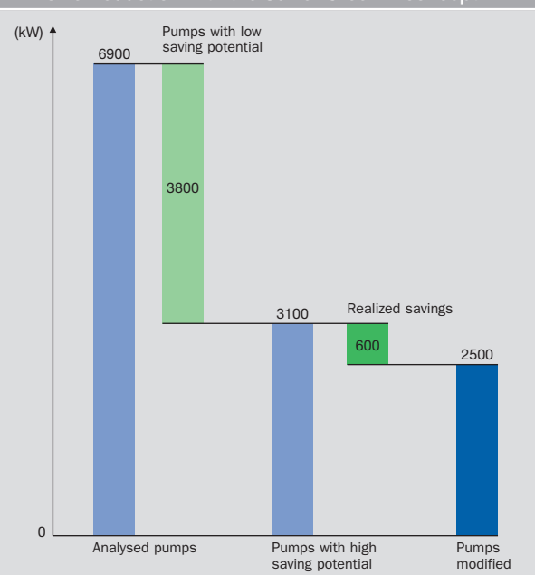
3 Power reduction with the Sulzer Green™ concept
